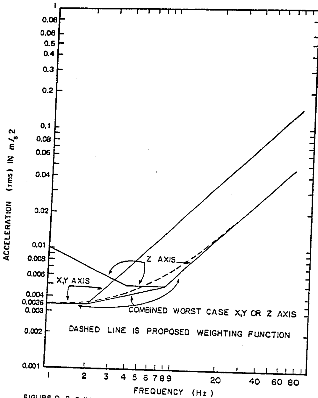
FIGURE D-2. Building vibration criteria for occupants in buildings. All curves are for hospital and critical working areas. See Table D-2 for proper scale factors.
